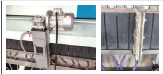
夹板清洗装置(选装自动) Cleaning device for pad(Optional Automatic)
