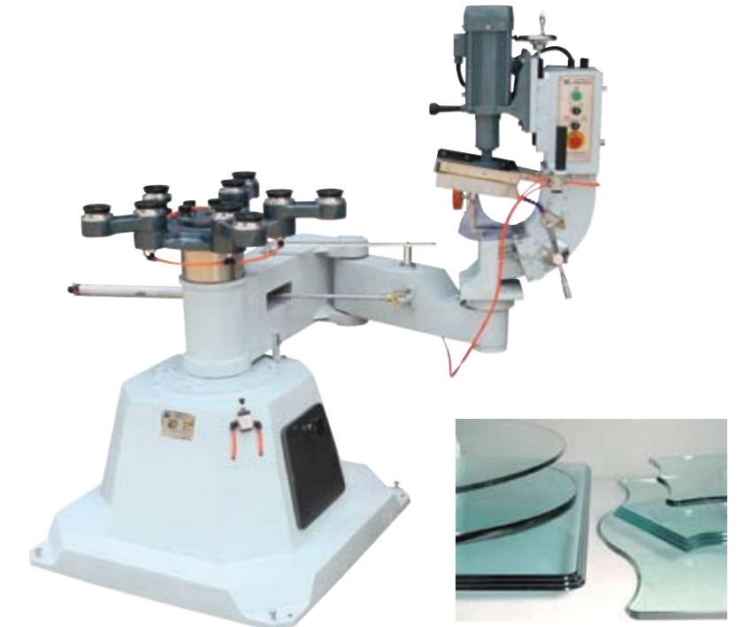
ZDYM1320 玻璃异形磨边机 Glass Shape And Beveling Machine
