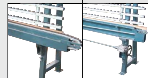
链条传送, 大玻璃更耐用 Chain transmission, large glass more durable 同步带传送, 小玻璃更准确 Synchronous belt transmission, small glass more accurate
