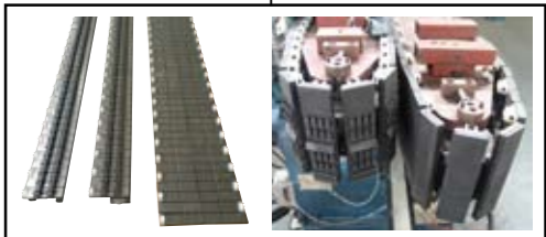
高频淬火达到55HRC硬度的夹板 55 HRC high-frequency quenching hardening Pad
